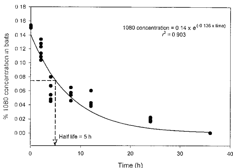
Fig. 3 Percentage of 1080 concentration remaining in Wanganui No. 7 baits after increasing lengths of time under flowing water (20 cm s -1 ). Also shown is the exponential decay relationship that displayed the best fit to the data, and the calculated half-life of 1080 under these experimental conditions. ( n = 6 for control samples, and samples collected at 2 and 4 h, and n = 4 for all other samples: some symbols are obscured by others.)
